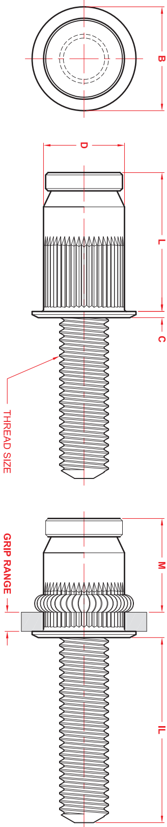
PART NUMBER EXAMPLE = 25C1IKSSV / .625 ( PART CODE + MATERIAL + FINISH / STUD LENGTH )
